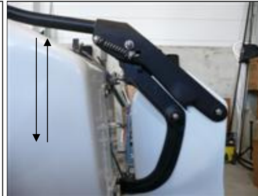
Step 6 Locking the rudders part 2 The rudder is now locked.
