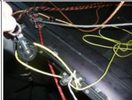
Jib Sheet Step 1 and 2
